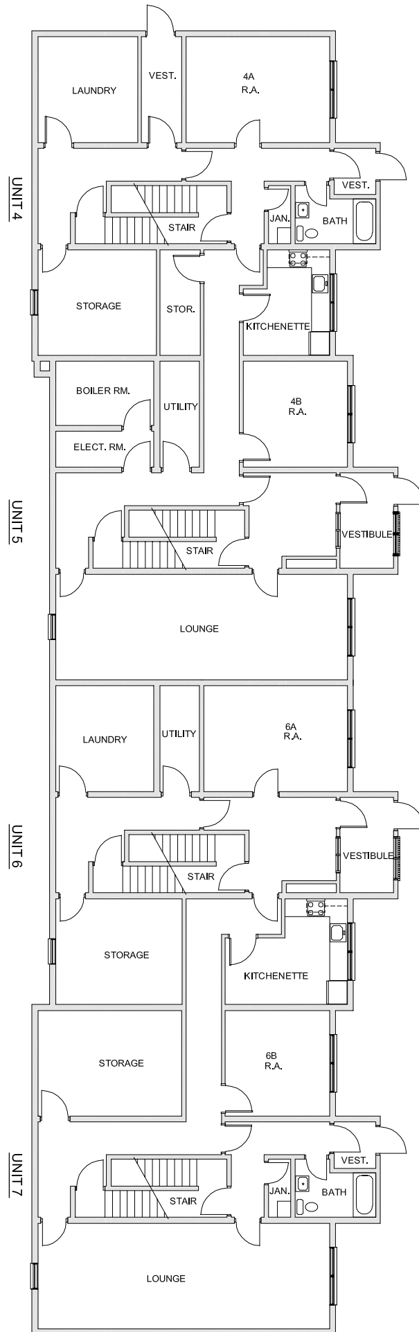
TOWNHOUSES - 4, 5, 6, 7 - BASEMENT LEVEL
